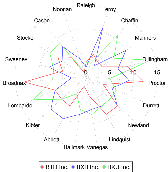
Radar Chart
